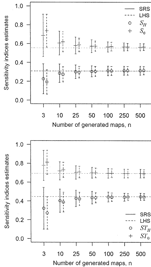
Figure 3. First order (top) and total order (bottom) sensitivity indices of input factors H ( \circ ) and \theta ( + ), depending on number n of generated maps and sampling strategy (SRS, LHS). Mean values with \pm s.d interval over 1000 replicas. The dashed lines show the analytical results from Tab. 1.
