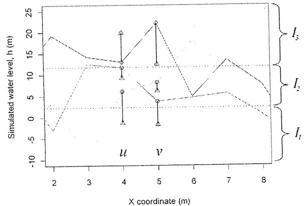
Figure 2. Three simulations of Gaussian random field H by Simple Random Sampling along a line of grid G . Water levels simulated by Simple Random Sampling ( \circ ) and Latin Hypercube Sampling ( \blacktriangle ) are given for two locations u et v . Vertical lines indicate the shift for individual sample elements; dotted horizontal lines indicate stratum boundaries.
